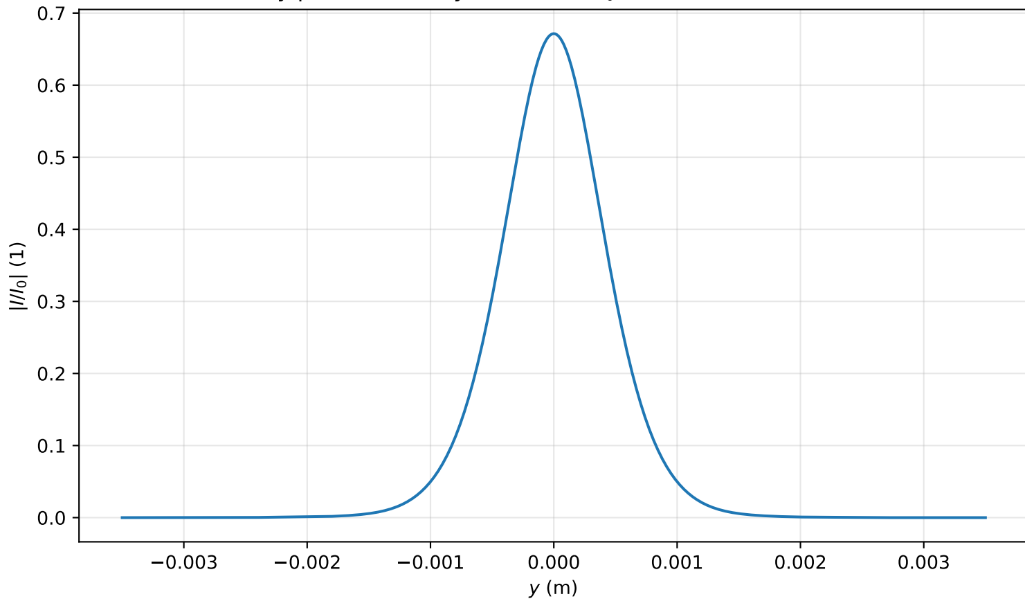
Intensity profile I(x = 0, y, z = 3.025)/I_0 , P_{in}=0.6P_{cr} , artificial time
